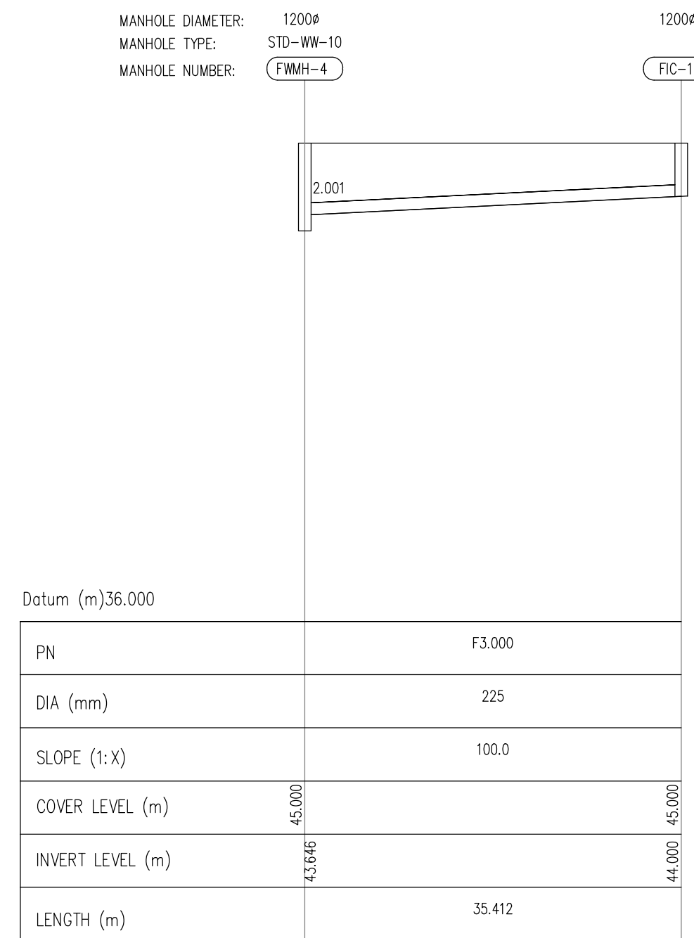
FOUL SEWER FROM FIC-1 TO FWMH-4 HORIZONTAL SCALE 1:500 VERTICAL SCALE 1:100
