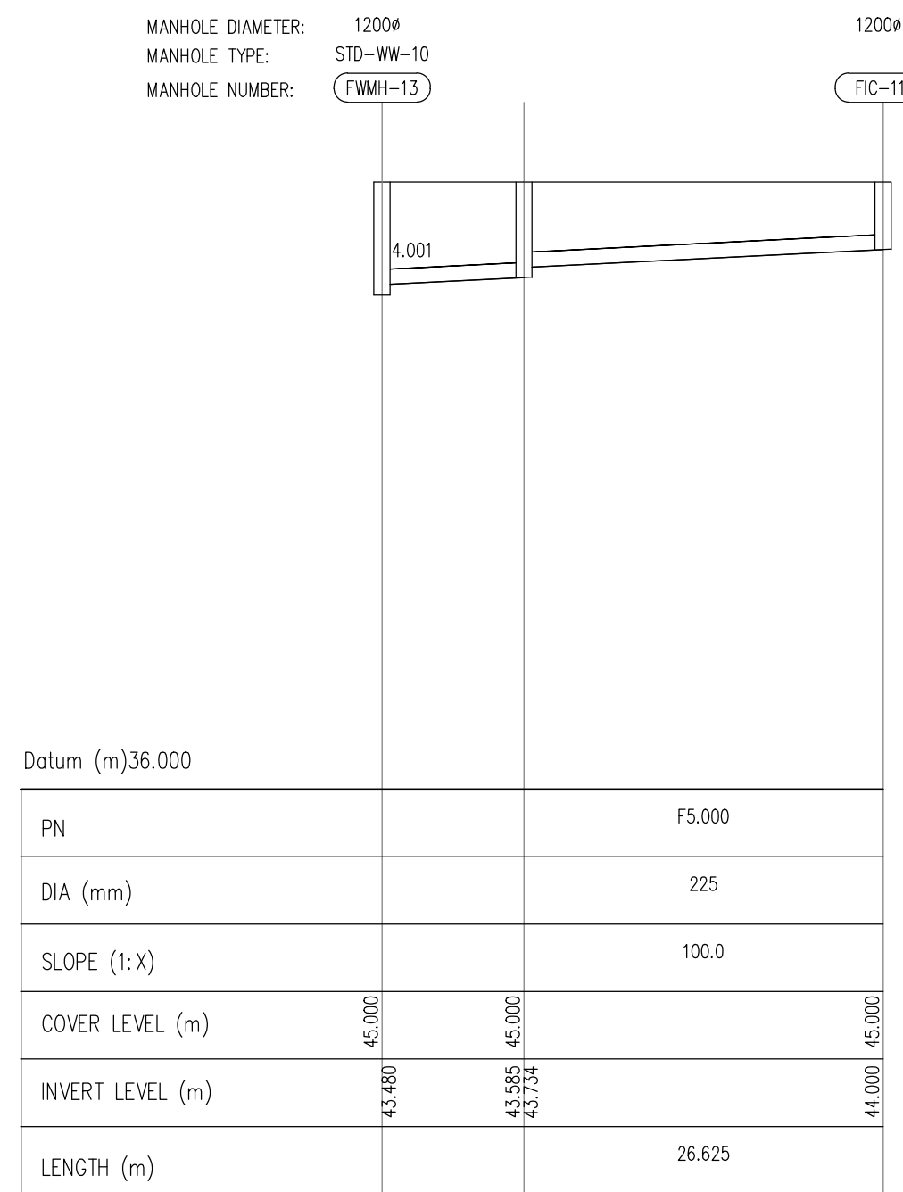
FOUL SEWER FROM FWMH-13 TO FIC-11 HORIZONTAL SCALE 1:500 VERTICAL SCALE 1:100
