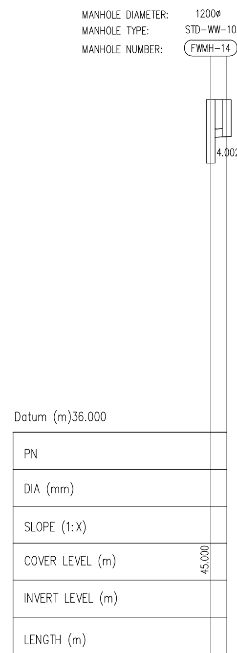
FOUL SEWER TO FWMH-14 HORIZONTAL SCALE 1:500 VERTICAL SCALE 1:100
