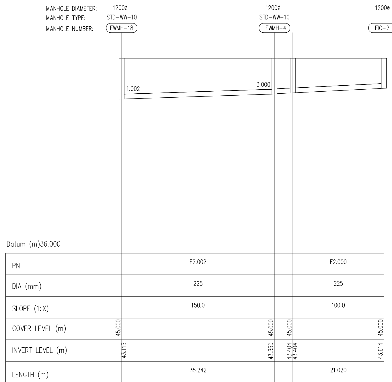
FOUL SEWER FROM SIC-4 TO FWMH-18 HORIZONTAL SCALE 1:500 VERTICAL SCALE 1:100
