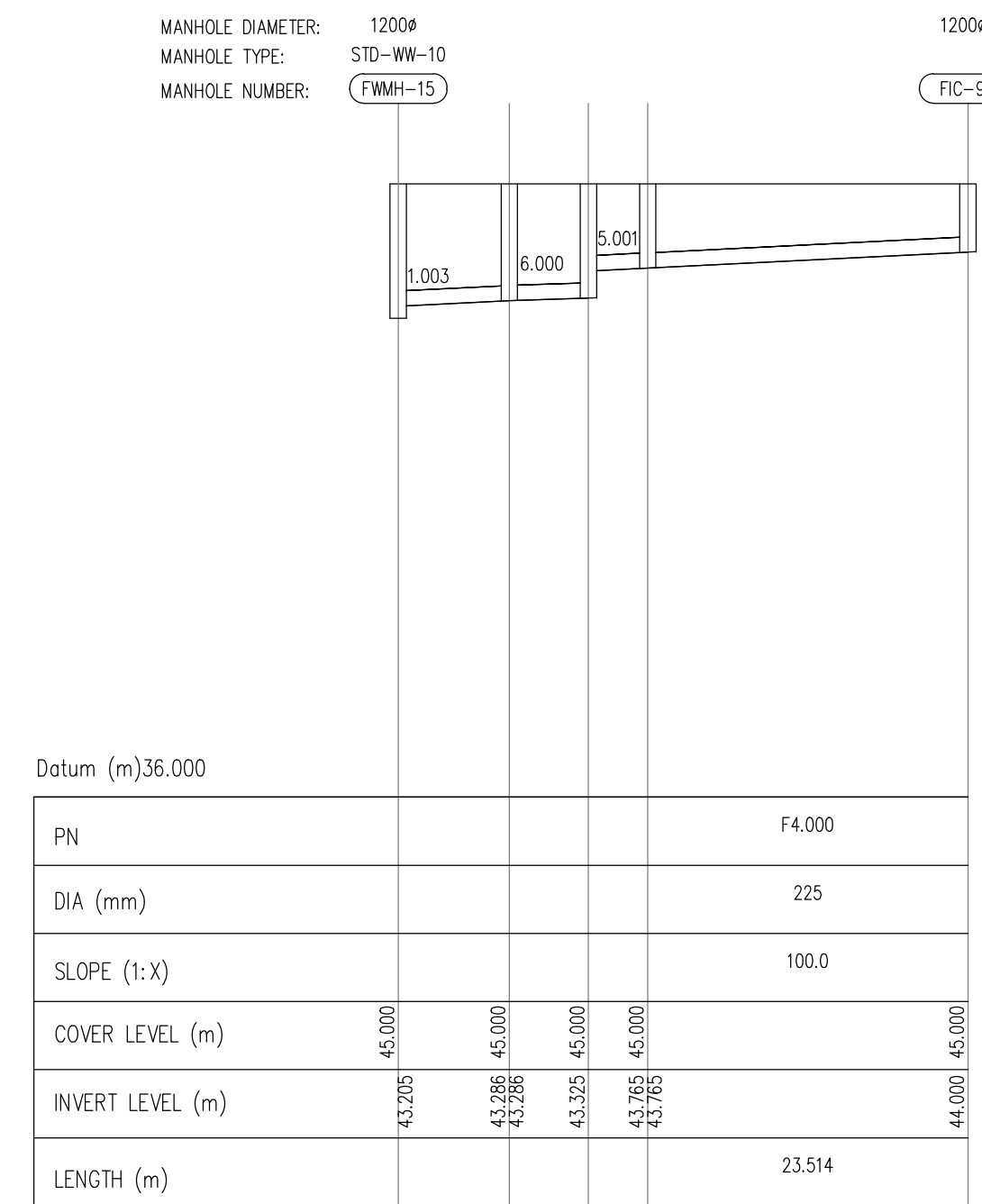
FOUL SEWER FROM FIC-9 TO FWMH-15 HORIZONTAL SCALE 1:500 VERTICAL SCALE 1:100
